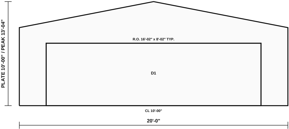
WEST ELEVATION | PLATE WALL 10'-00"
