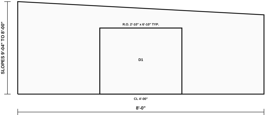
WEST ELEVATION | WALL 9'-04"
