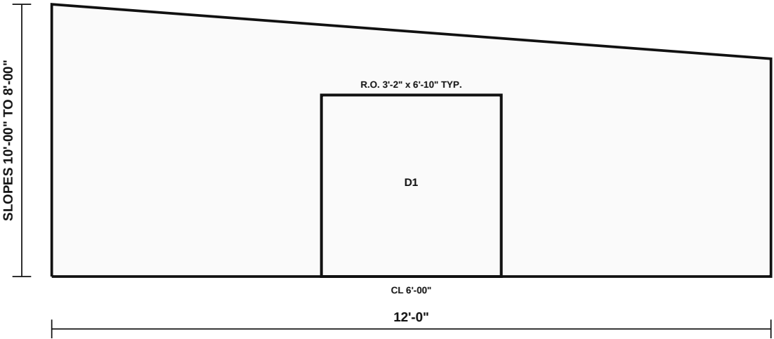
WEST ELEVATION | WALL 10'-00"
