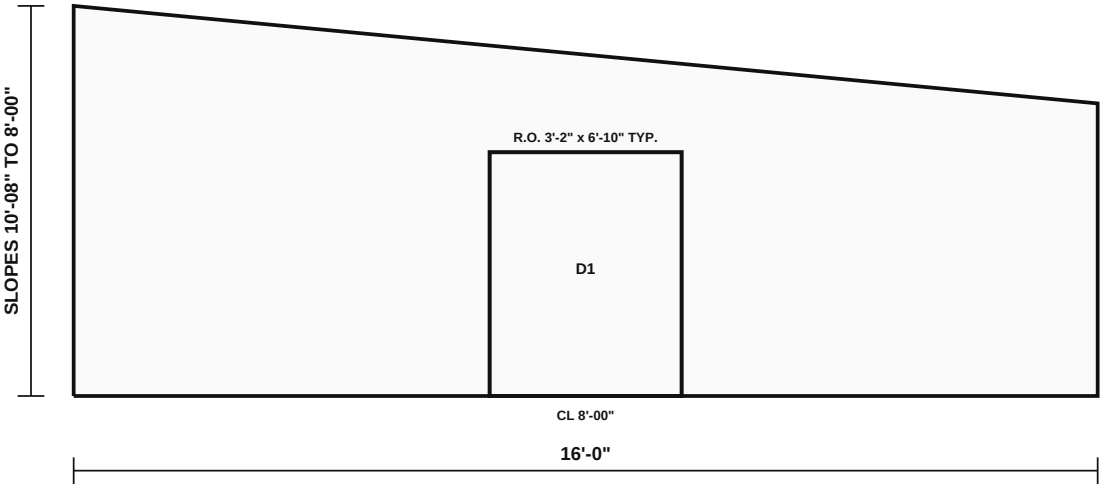
WEST ELEVATION | WALL 10'-08"
